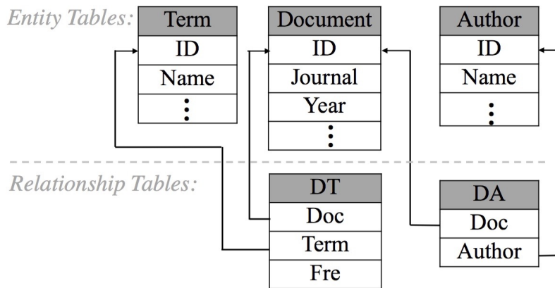
Figure 1: PubMed database schema . Relationship tables DT and DA have reference keys pointing to entity tables Document , Term and Author .
