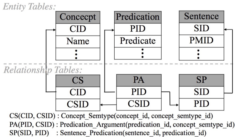
Figure 7: SemmedDB database schema . CS , PA and SP are relationship tables while the others are entity tables.
